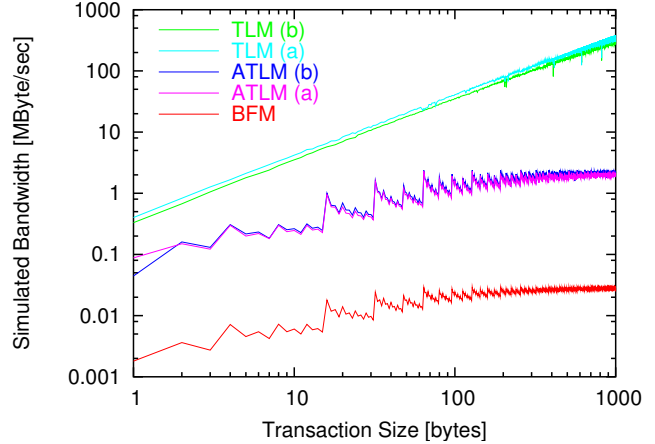
Figure 4. Simulated bandwidth.
