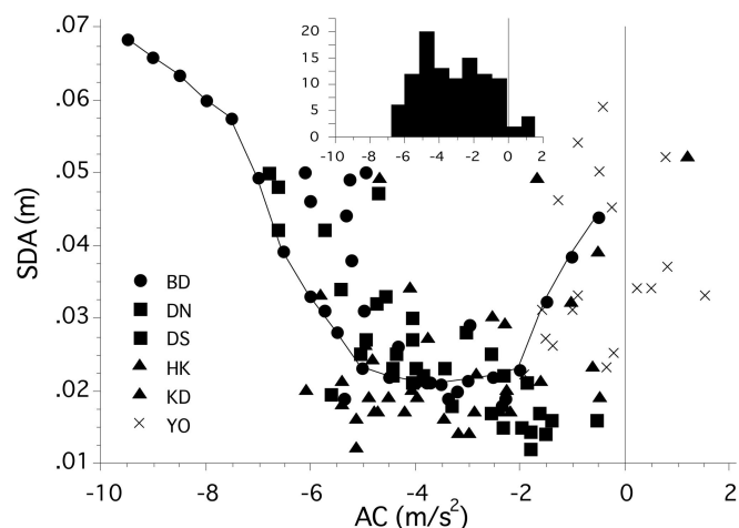
FIGURE 3. Standard deviations of ball amplitude ( SDA ) plotted against acceleration at impact ( AC ) from all subjects and all conditions in experiment 1. Each data point is a trial mean. The different symbols denote the six subjects. The solid line represents the predicted function of variability calculated from a Lyapunov stability analysis. The inserted figure is a histogram of the AC values from all subjects and conditions.
