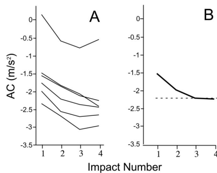
FIGURE 6. Acceleration of the racket at impact as a function of the impact number from experiment 3. Impact 1 is the impact following the perturbation. Impacts 2, 3, and 4 denote the following impacts. (A) Each line corresponds to one subject. (B) The solid line represents the average across all six subjects. The dashed line is the overall trial average from the unperturbed trials.
