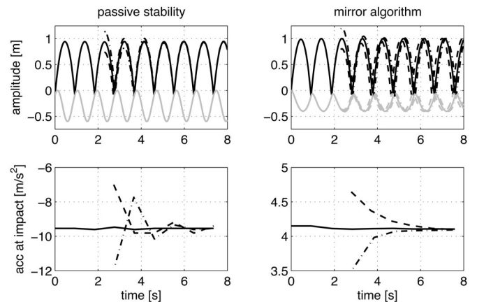
FIGURE 2. Simulation of the trajectories of ball and racket for the regime with passive stability (left panels) and with the mirror algorithm (right panels). In both simulations, perturbations were applied in cycle 3. The two top panels show the simulated trajectories. The dashed lines represent the two perturbed trials, whereas the solid line corresponds to the unperturbed trial. The two bottom panels show the corresponding accelerations of the racket at impact AC .
