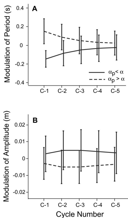
FIGURE 8. Modulation of racket period (A) and amplitude (B) as a function of cycle number in the perturbed trials. The data of all subjects are averaged. The vertical bars denote the standard deviations. The dashed lines correspond to those trials where the perturbed coefficient of restitution \alpha_p was greater than \alpha = 0.50 . The solid lines correspond to those trials where the perturbed coefficient of restitution \alpha_p was smaller than \alpha = 0.50 .
